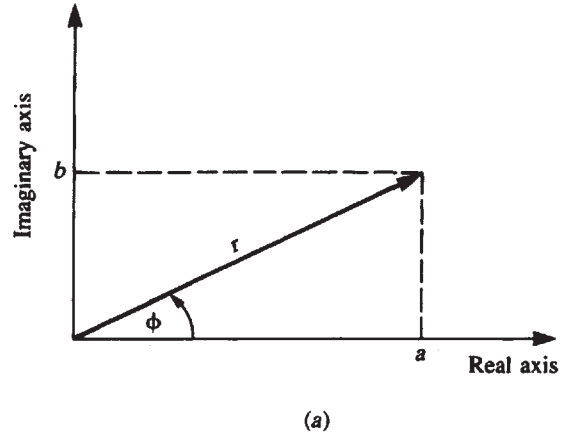
Figure 1.4 (a) Representation of a complex number as a point in the complex plane in both cartesian (a, b) and polar (r, \phi ) coordinates. (b) A succession of values of the complex numbers (1 + i)^n . The radius vector rotates and stretches as higher powers are taken.
