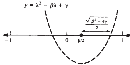
Figure 2.10 For stability of a second-order system such as (23), both eigenvalues corresponding to roots of the characteristic equation y = \lambda^2 - \beta\lambda + \gamma must lie within the interval (-1, 1) .
