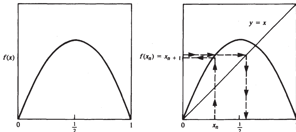
Figure 2.4 The parabola y = f(x) and the line y = x can be used to graph the successive values of x_n , n = 0, 1, 2, \dots . This is known as the cobwebbing method (see Figure 2.5).
