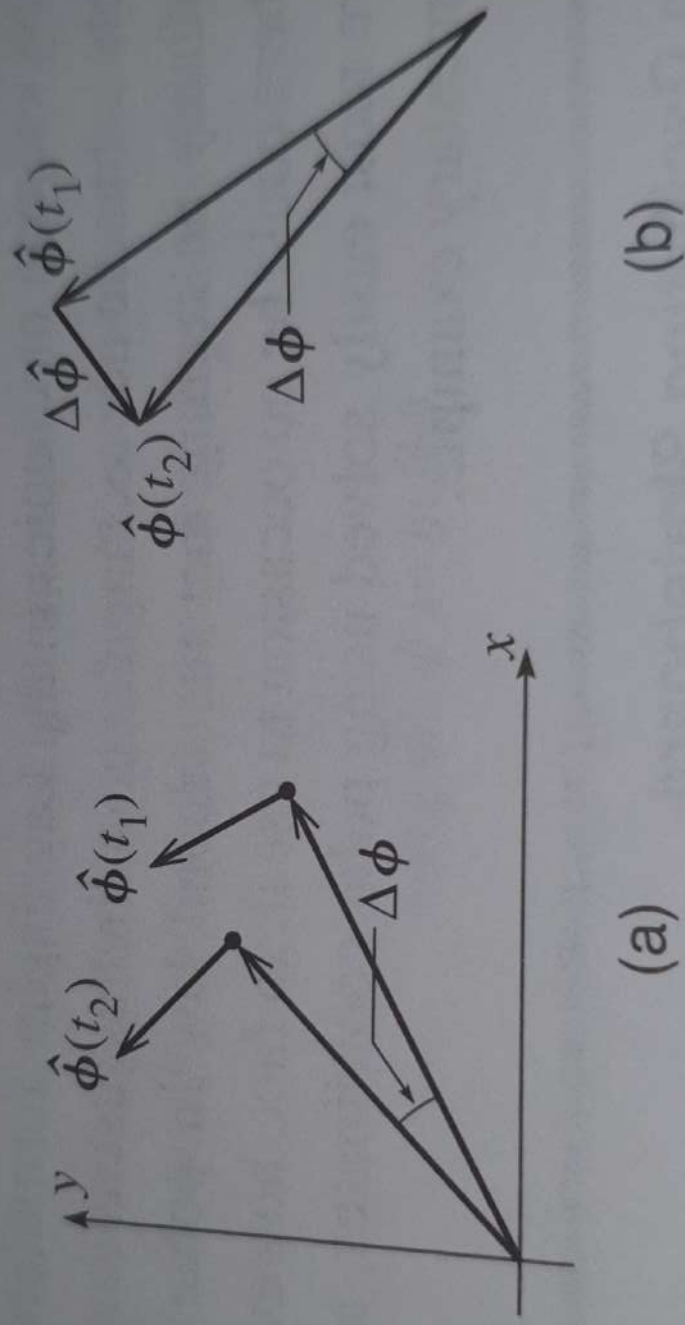
Figure 1.13 (a) The unit vector \hat{\phi} at two successive times t_1 and t_2 . (b) The change \Delta\hat{\phi} .
